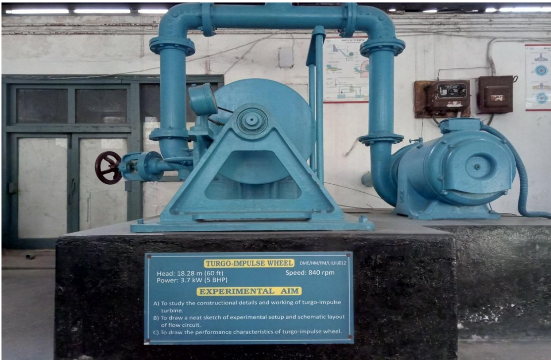
Fig.2: Turgo Impulse Wheel
